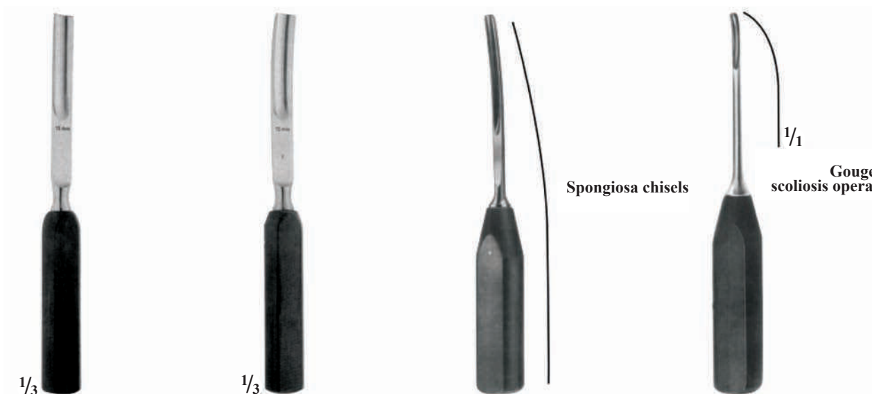
LEXER Straight 09-298-250 0.5 cm 09-299-250 1.0 cm 09-300-250 1.5 cm 25 cm Tip size
